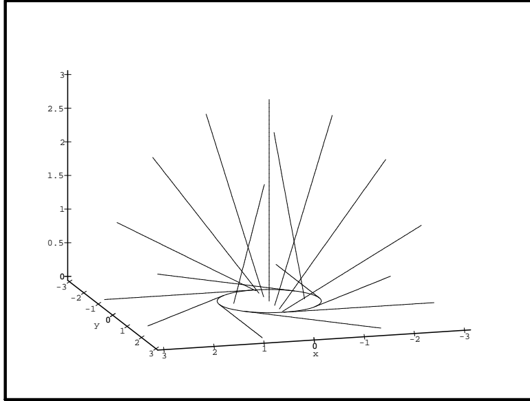
Figure 7.1: Incoming light paths for the Kerr solution I — view from above. The paths terminate over a central disk in the z = 0 plane.
